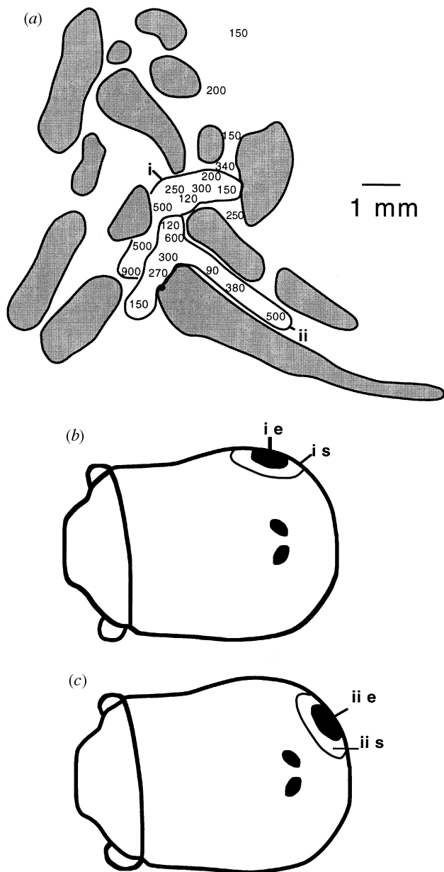
Figure 7. (a) A patch of electrosensory cortex in the platypus. The shaded areas represent regions of high CO density. These regions contain neurons responsive to mechanosensory stimulation. In the enclosed white areas, the individual numbers represent electrode penetrations at which neurons responded to electrosensory and mechanosensory stimulation. The numbers themselves are the threshold in \mu\text{V cm}^{-1} for neurons at those sites. The receptive field location for neurons at all of the sites within the enclosed white area was the same. For instance, the electrosensory field for neurons in the 'i' enclosed region is drawn in (b) and is indicated as 'ie'. The somatosensory receptive field is indicated in (b) as 'is'. (c) The same relationship exists for neurons in the 'ii' enclosed area. Note that the electrosensory receptive field and somatosensory receptive field are completely overlapping, although the electrosensory receptive field is smaller. This figure is redrawn from Krubitzer et al. (1995).
